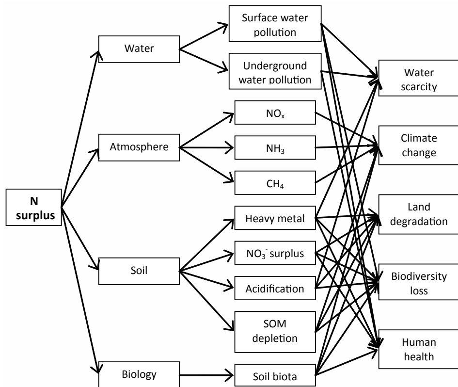
Fig. 1 The multifaceted and complex consequences of N surplus in agroecosystems. It is worth noting that N surplus is not the only driver of agroecosystem degradation. Other unsustainable practices, such as deep tillage and heavy application rate of biocides, could also add to specific consequences, and enhance soil degradation in the long run.
