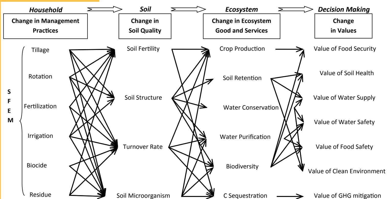
Fig. 3 A comprehensive and hierarchical framework of SOM Friendly Ecosystem Management (SFEM) and its linkage with soil, ecosystem, and their valuing for decision making. The SFEM will only succeed when all the aspects of the practices are handled properly.
