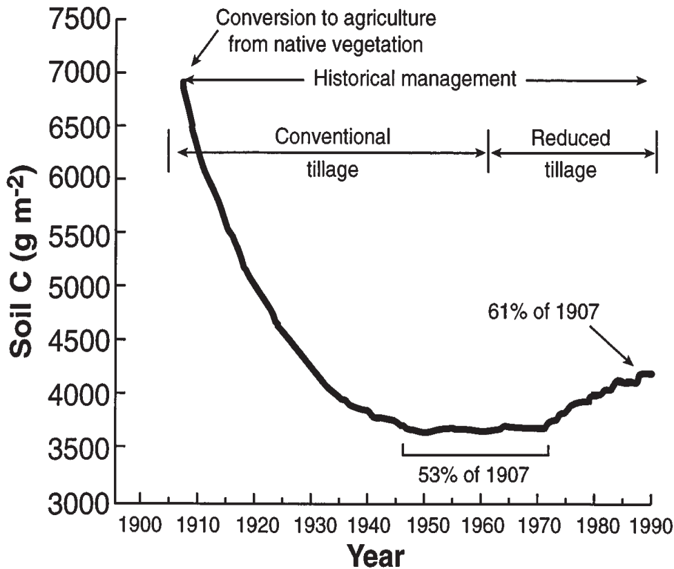
Fig. 2 Simulated total soil carbon (for soil depth of 0 to 20cm) changes for the central U.S. corn belt. Points at which soil carbon was 53 and 61% of concentration at conversion to agriculture (in 1907) are indicated (Adapted from Matson et al. 1997).
