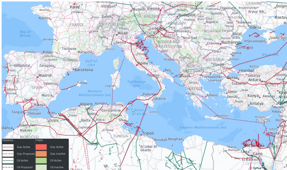
Figure 55. Active and proposed oil and gas pipelines in the Mediterranean. Source: Clarksons Research OIN; map retrieved on 09.06.2020.
