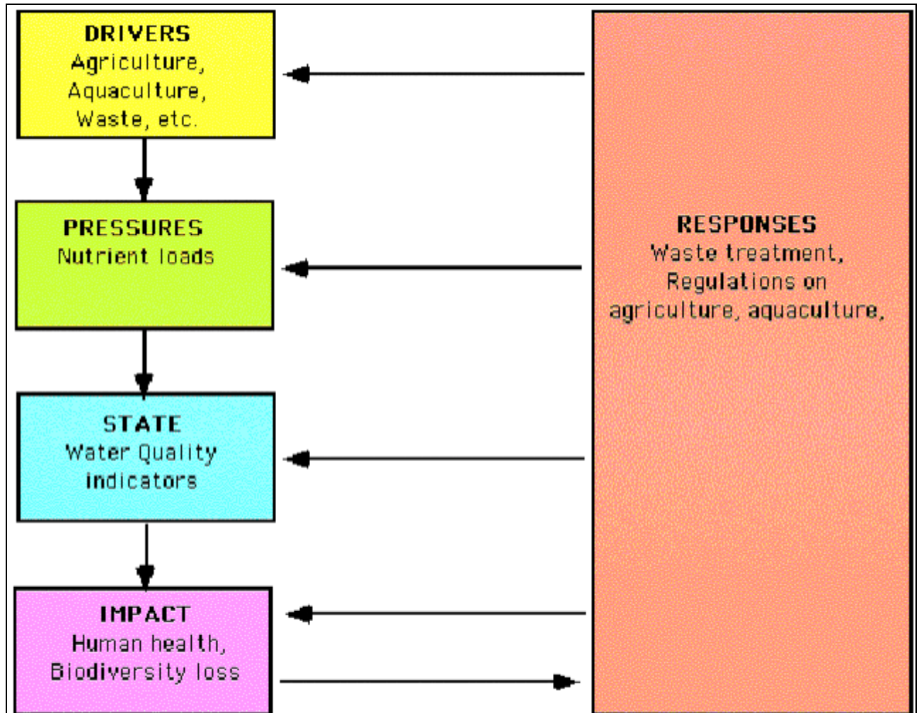
Fig. 4 The DPSIR Framework applied to eutrophication
