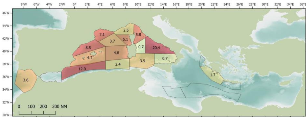
Figure 4. 44 : Sperm whale acoustic densities (individuals per 1000 km²) derived for each block surveyed by the Song of the Whale team. Empty blocks represent those areas where no on-track detections were made. Source: ACCOBAMS, 2021b.
