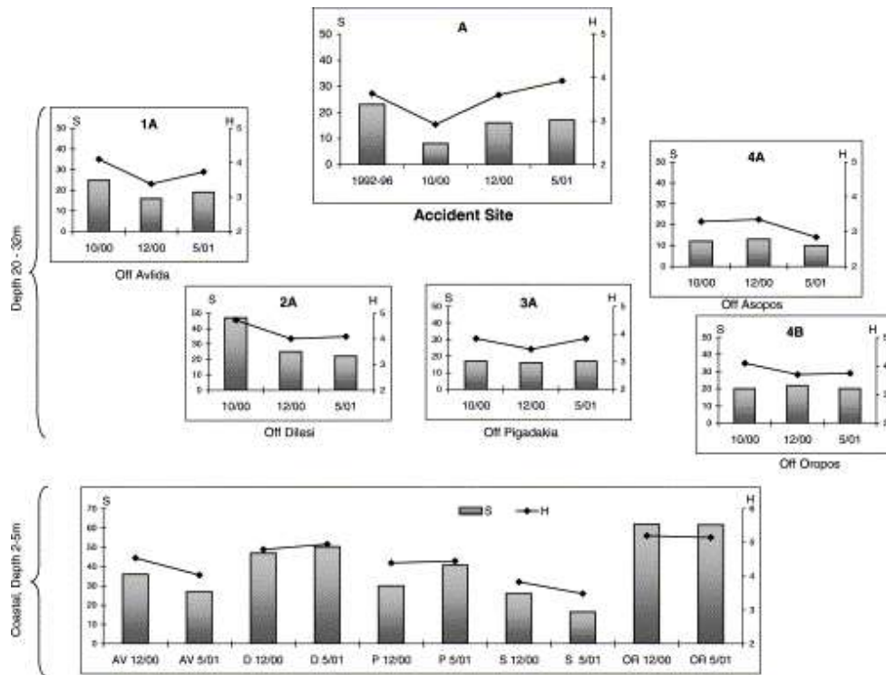
Figure 31. Temporal changes in the ecological indices ( S : number of species, H : community diversity) at the sampling sites over the 8-month study period. The position of the plot frames in the figure represents the geographical orientation of the sampling sites in relation to the accident site. Source: Zenetos et al. (2004)
