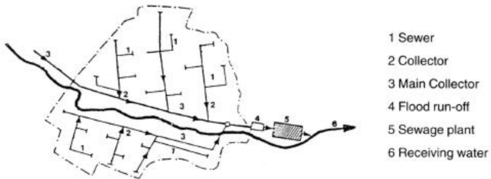
Figure 3.4: Scheme of a sewage network
