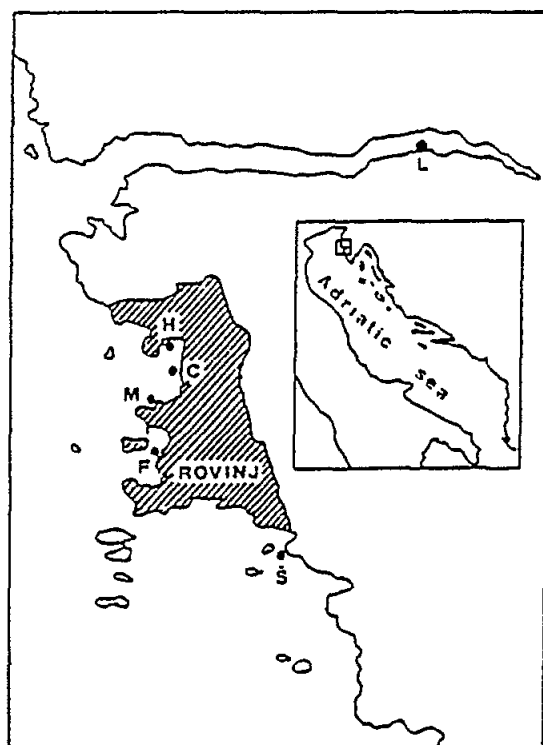
Fig. 1 Location of sampling sites in the Rovinj sea area, Northern Adriatic. Š: Škarabe-site; F: Factory-site; M: Market-site; C: Cannery-site; H: Hospital-site; and L: Lim-site.
