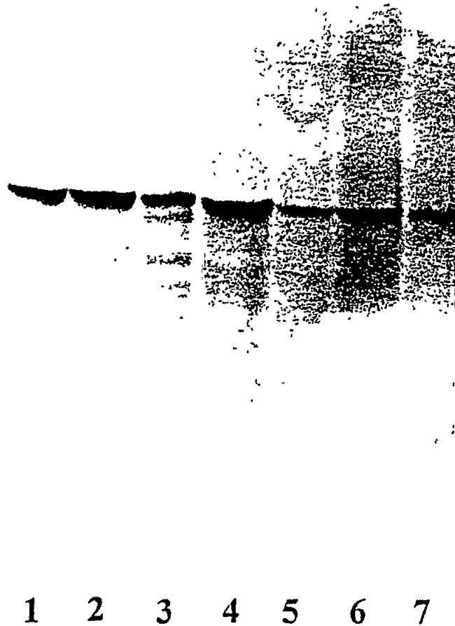
Fig. 8 Immunoblot of liver microsomes obtained from control and BNF-treated gilthead seabreams. Following electrophoretic transfer, the nitrocellulose sheet was incubated with 3% BSA for 75 minutes to reduce the nonspecific binding. The blot was then allowed to react with polyclonal antibodies (produced against purified CYP1A1 from BNF-treated cod) for 1.5 h at room temperature with constant shaking. Then the blot were incubated with second antibody (Anti-Rabbit IgG-Alkaline Phosphatase Conjugate) in 1% BSA in TBST for 1 h. Finally, blots were incubated with substrate solution as described by Ey and Ashman (1986) to visualize the specifically bound antibodies. Lanes 1-4 are liver microsomes from BNF-treated gilthead seabreams and Lanes 5-7 are control fish liver microsomes
