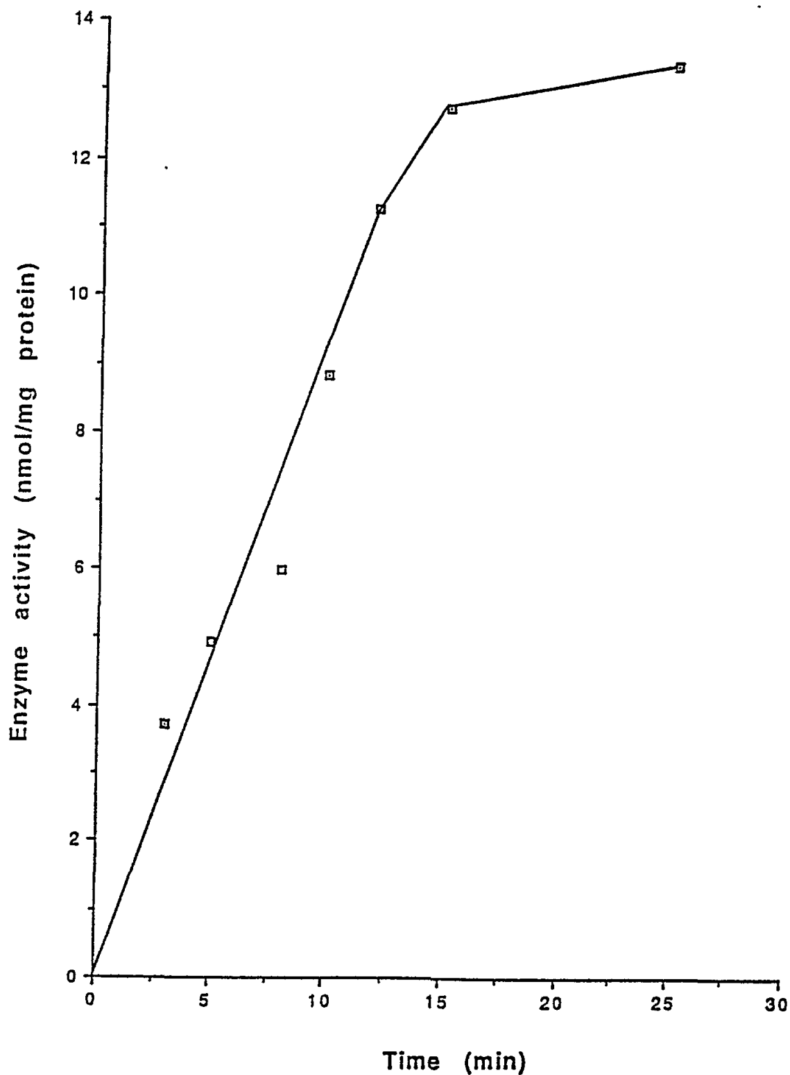
Fig. 1 Effect of incubation time on gilthead seabream liver microsomal 7-EROD activity. The reaction mixture contained 200 \mu g microsomal protein obtained from B(a)P treated fish liver. The reaction was carried out 25°C as described in Materials and Methods. The points are the means of two sets of duplicate determinations
