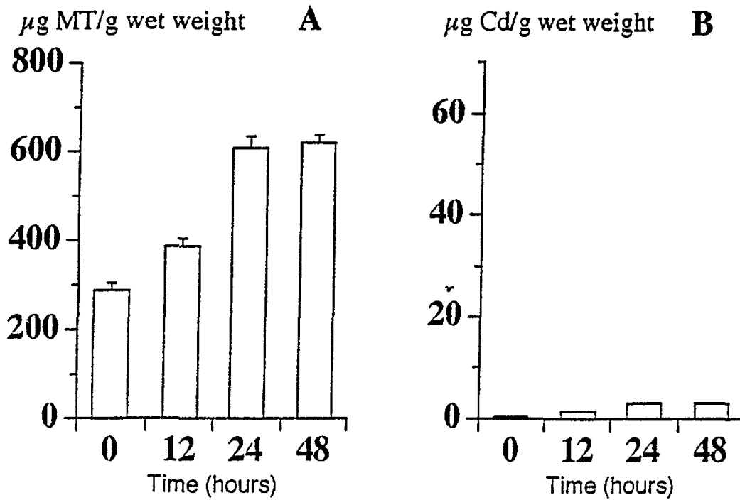
Fig. 3 MT concentrations (A) and cadmium content (B) in Artemia after 0, 12, 24, and 48 hours of exposure to 10 \text{ mg Cd l}^{-1}
