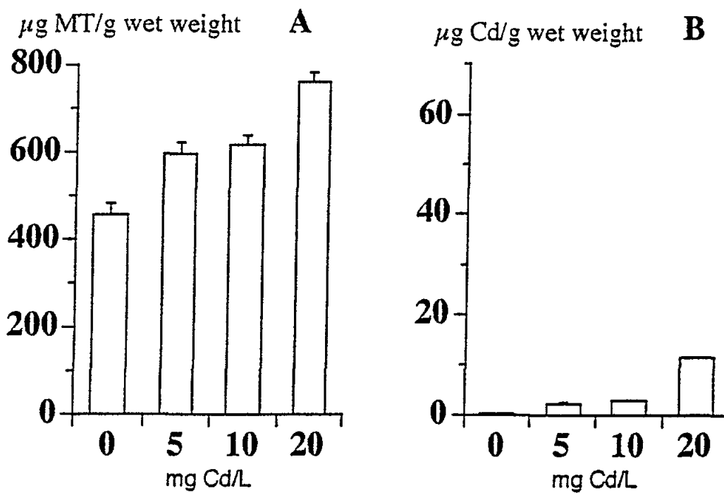
Fig. 4 MT concentrations (A) and cadmium content (B) in Artemia after 48 hours of exposure to 0, 5, 10, and 20 \text{ mg Cd l}^{-1}
