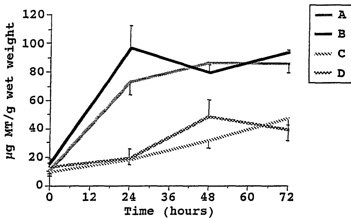
Fig. 8 MT concentrations at different times from the start of the experiment. Values represent the means \pm S.D. (n= 3). Error bars indicate S.D.
