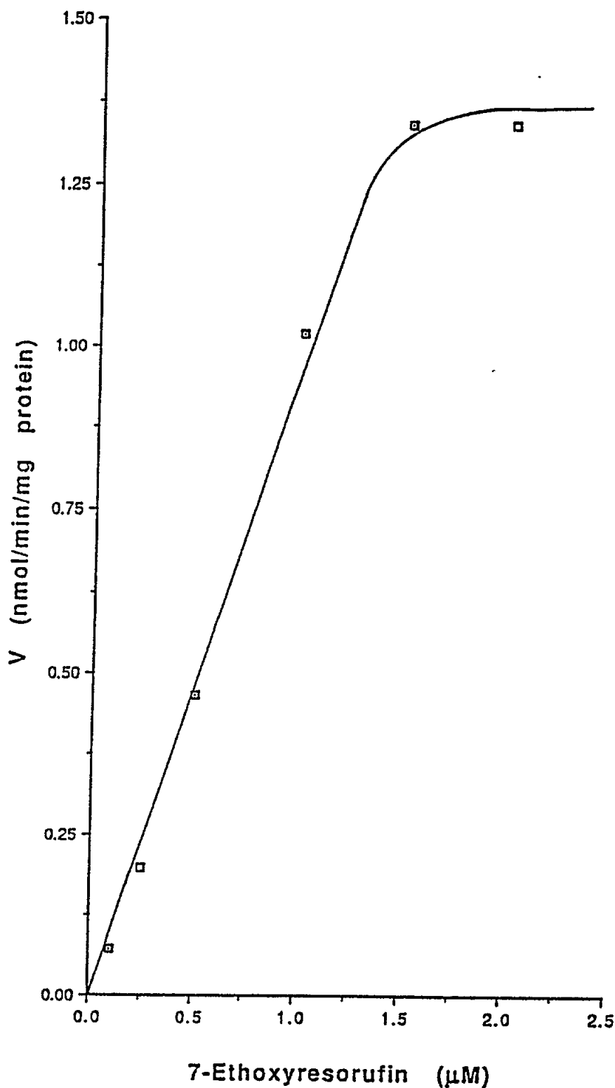
Fig. 3 Substrate saturation curve for 7-EROD of gilthead seabream liver microsomes. Incubation mixture contained 7-ethoxyresorufin concentrations ranging from 0.1 \mu M to 2.0 \mu M, 0.5 mM NADPH, 100 mM phosphate buffer, pH 7.8 containing 100 mM NaCl, 200 \mu g liver microsomal protein obtained from B(a)P-treated fish and 1.2 mg BSA in a final volume of 1.0 ml. The values are averages of two different sets of data each of which was a duplicate determination
