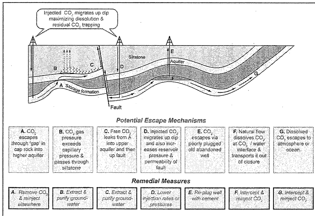
Figure 4 Escape mechanisms and remedial measures (IPCC, 2005).
