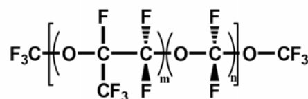
Figure 6-6. Structure of a perfluoropoly-methylisopropyl ether.
