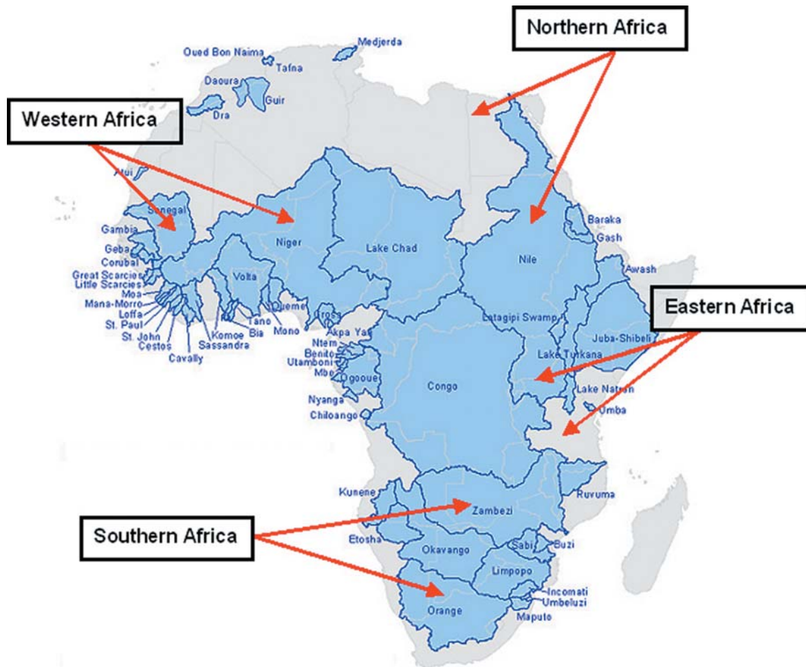
Figure 3.1: International river/lake basins of Africa (Transboundary Freshwater Dispute Database, 2000)
