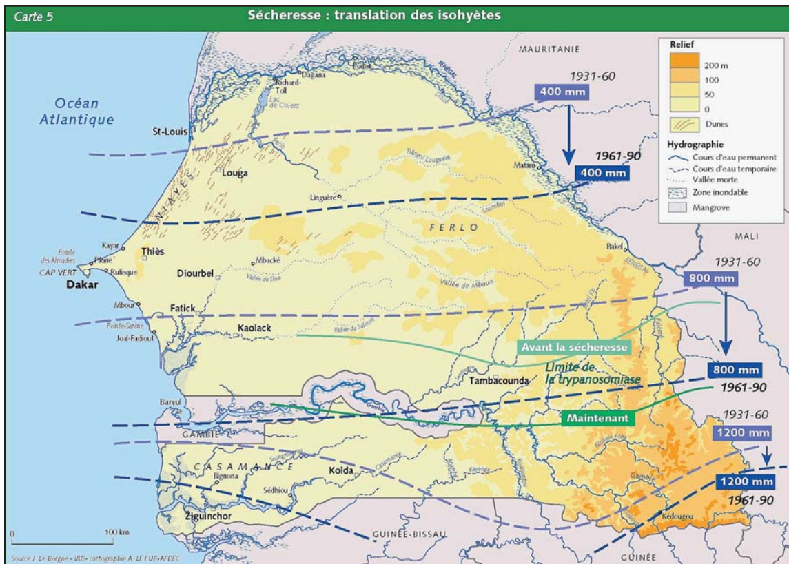
Figure 3.15: Southward shift of isohyets in the Senegal River Basin
