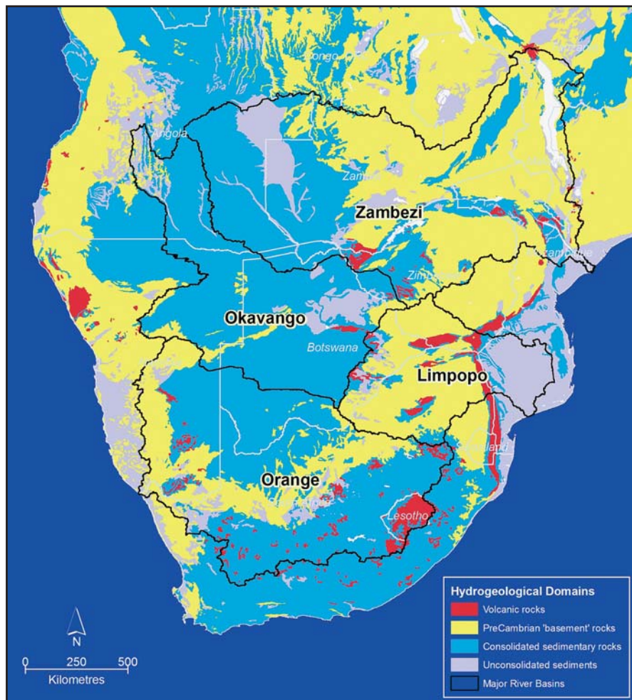
Figure 3.4: Hydrolithological domains of Southern Africa
