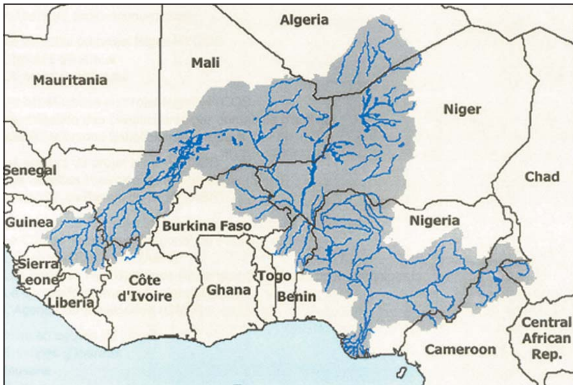
Figure 3.16: Niger River Basin
