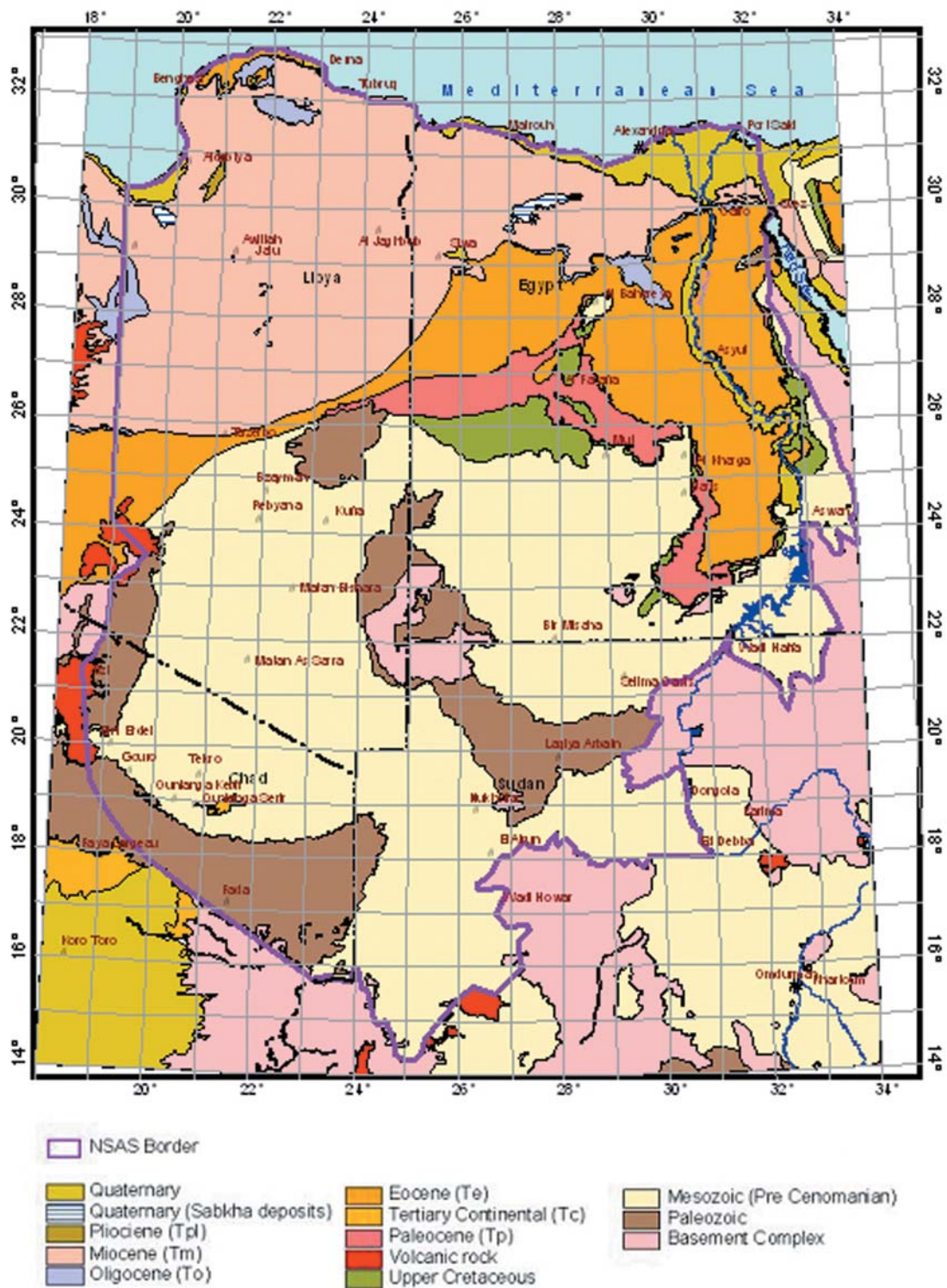
Figure 3.24: Nubian Sandstone Aquifer System (CEDARE, 2001)
