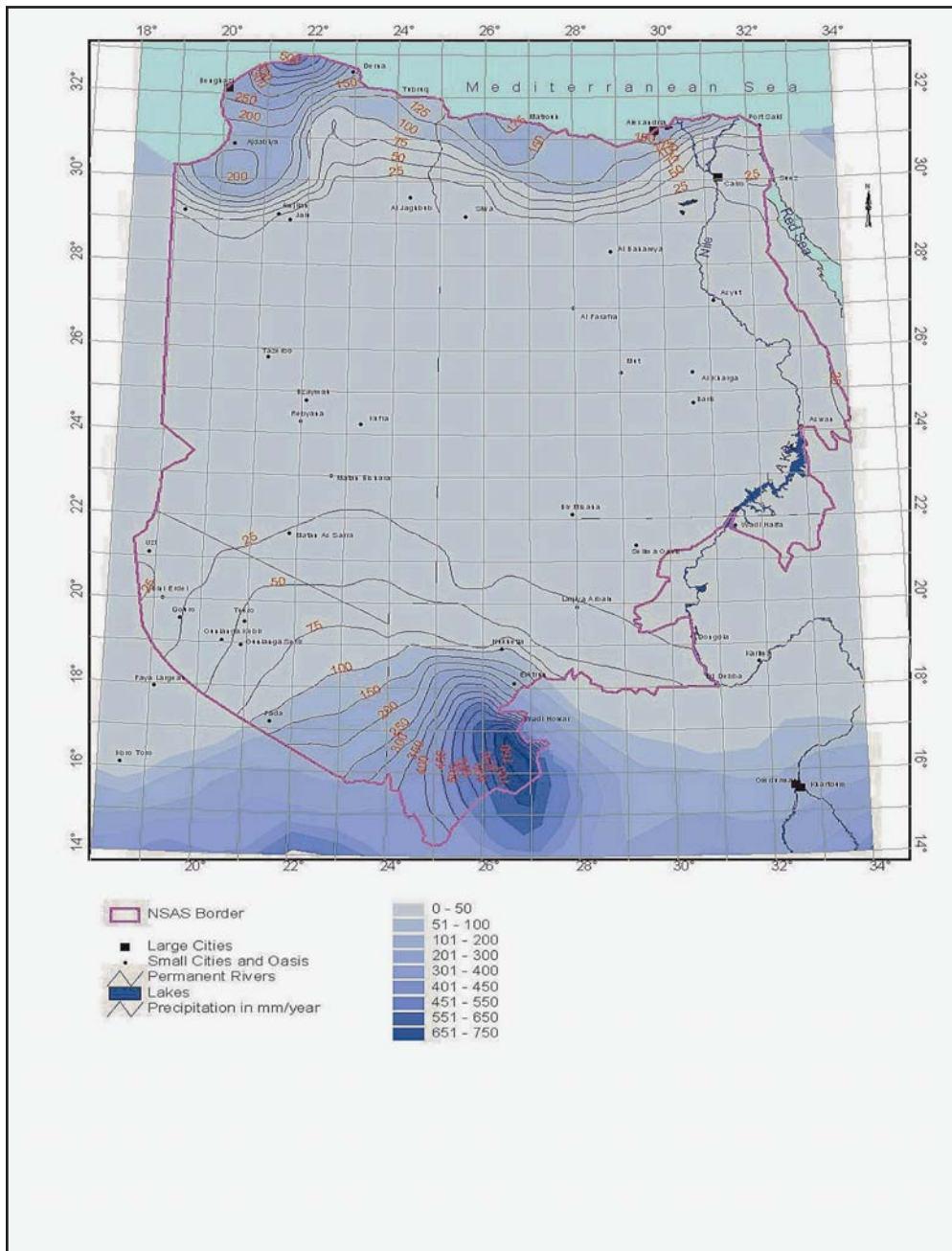
Figure 3.25: Rainfall distribution on the fringes of the Nubian Sandstone Aquifer System
