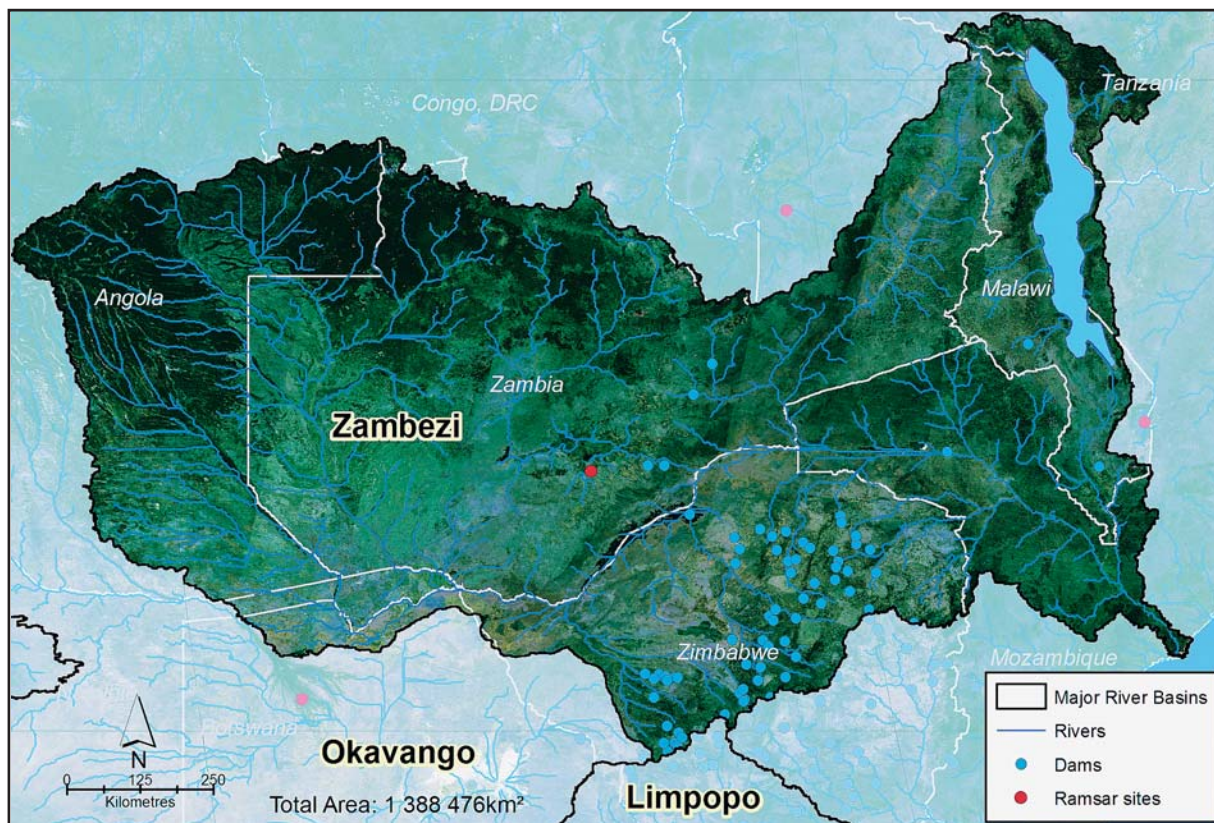
Figure 3.5: Zambezi River Basin
