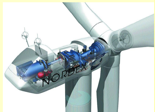
Internal view of a large grid-connected wind turbine
