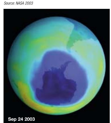
Figure 3: The 2003 ozone hole over Antarctica dark blue denoting high levels of ozone depletion was very large, close to the all-time record.
