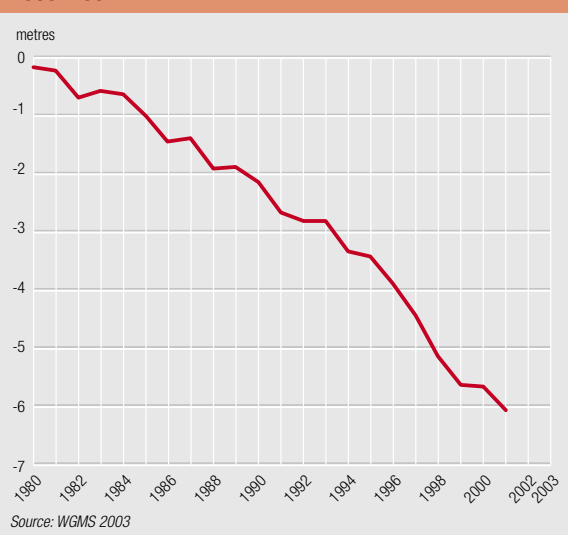
Figure 6: Glacier mass balance (metres), global average, 1980–2001
