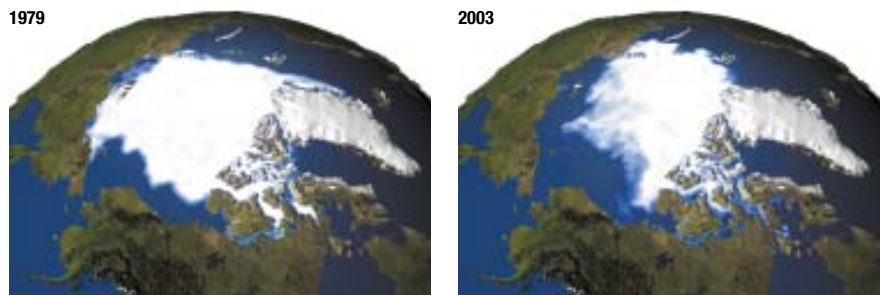
Figure 1: Dramatic changes in Arctic sea ice since 1979. The loss of Arctic sea ice may be caused by warming Arctic temperatures that result from greenhouse gas build-up in the atmosphere.
