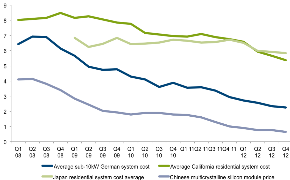
FIGURE 38: SMALL PV SYSTEM COST IN JAPAN, GERMANY AND CALIFORNIA, $/W
