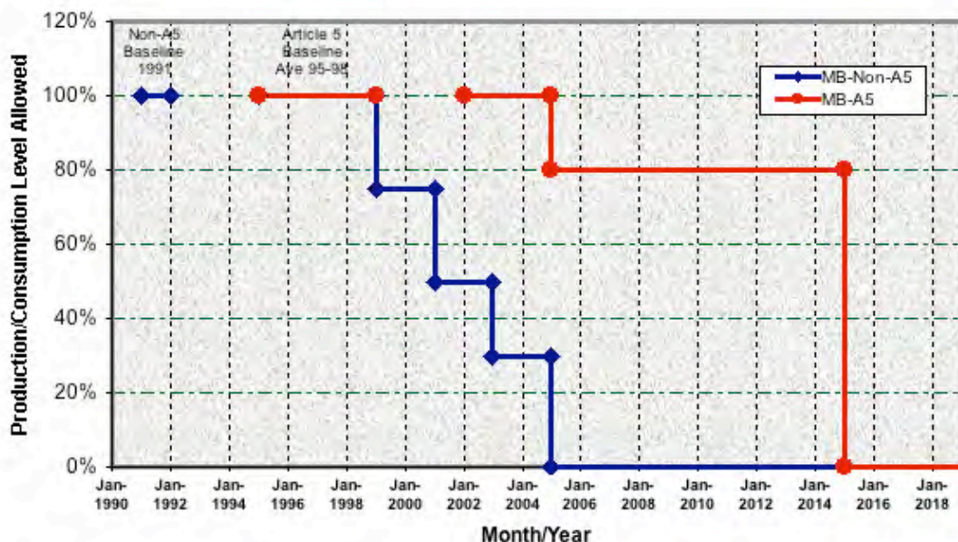
Methyl bromide (Annex E) Production/Consumption Reduction Schedule
