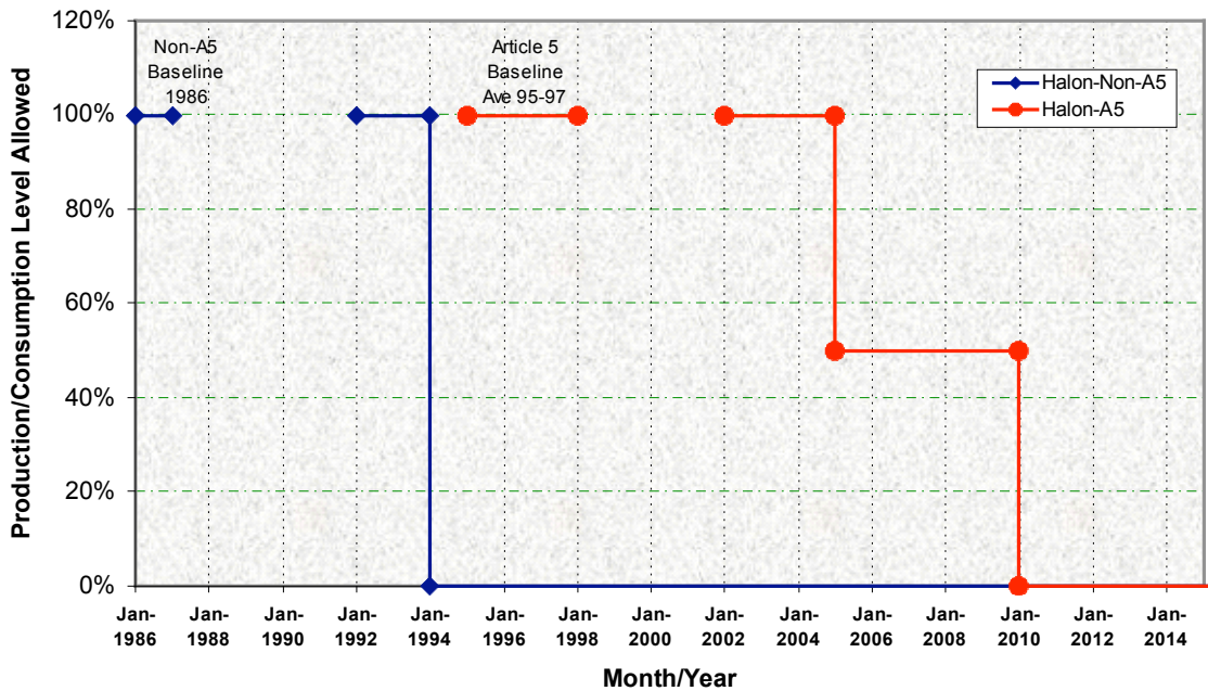
Halon (Annex A/II) Production/Consumption Reduction Schedule
