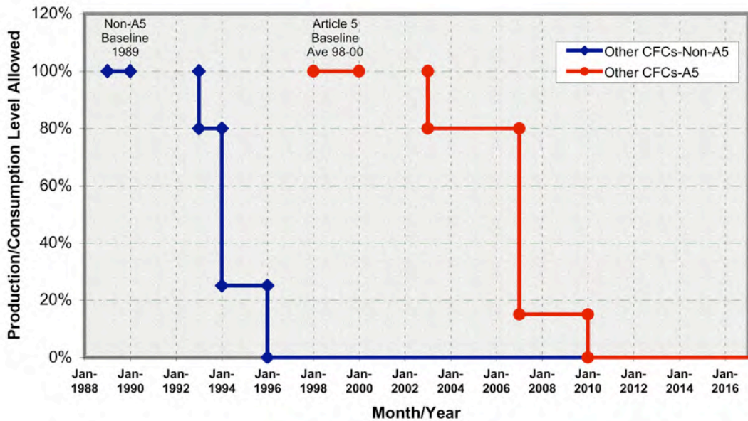
Other CFCs (Annex B/I) Production/Consumption Reduction Schedule
