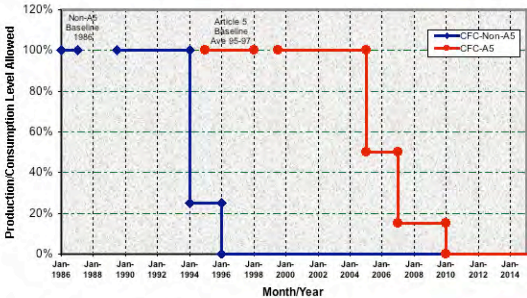
CFCs (Annex A/I) Production/Consumption Reduction Schedule
