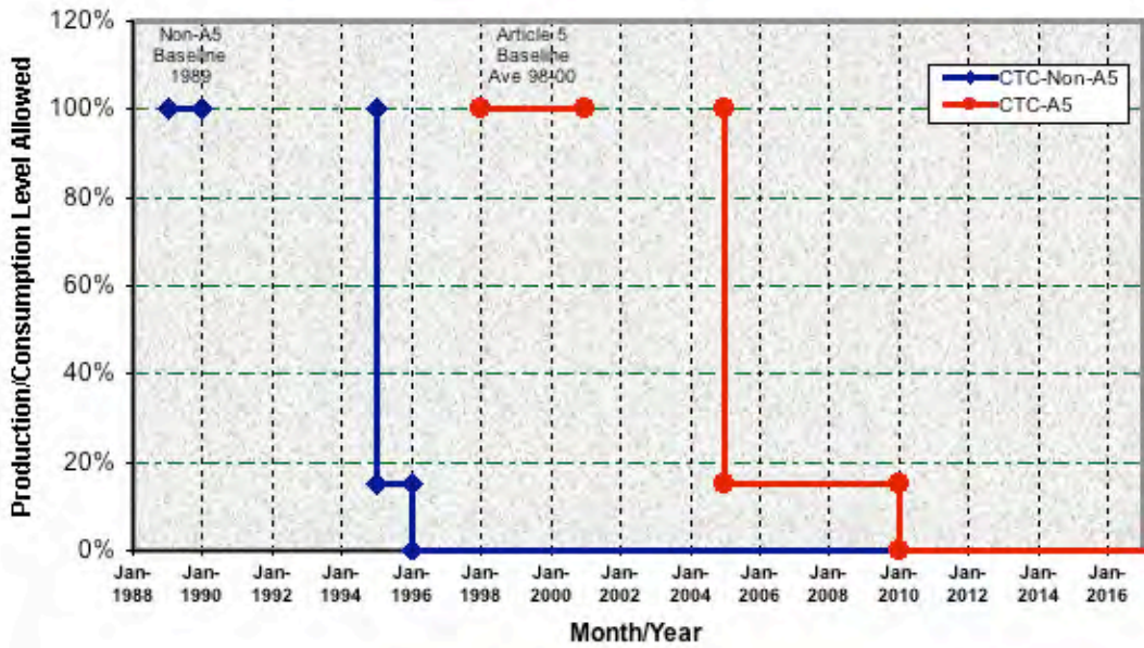
Carbon tetrachloride (Annex B/II) Production/Consumption Reduction Schedule
