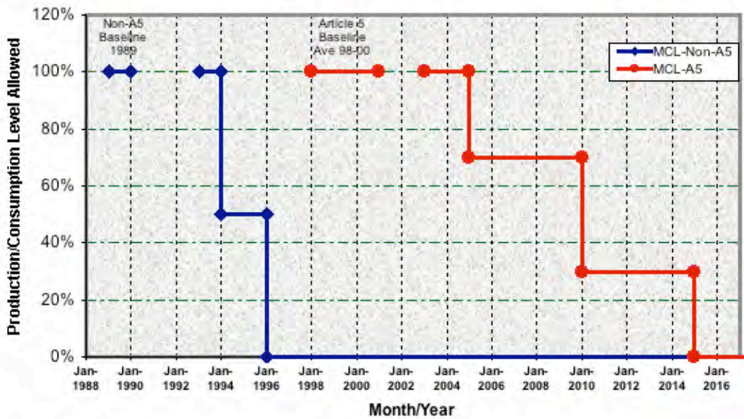
Methyl chloroform (Annex B/III) Production/Consumption Reduction Schedule
